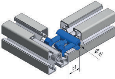
BOLZENVERBINDER [D]
